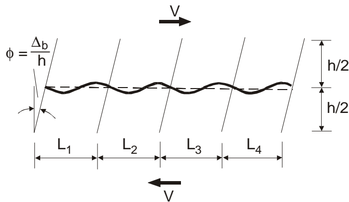
Fig. 1. Story drift due to girder flexure
